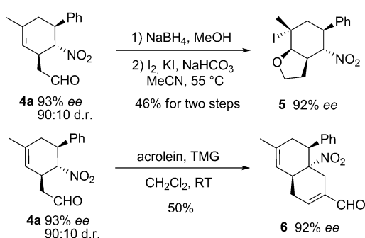
Scheme 3. Synthetic transformations of Diels–Alder adduct 4a . TMG = tetramethylguanidine.
